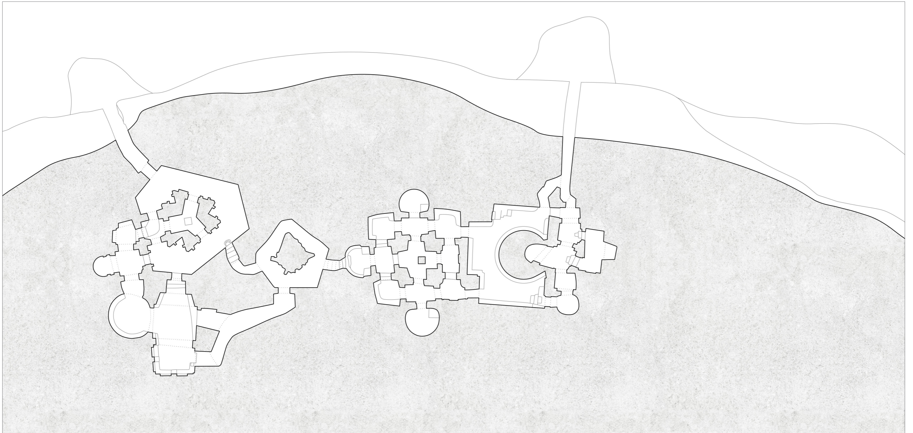
Dagmawi Lalibela (Ambager Complex) Ground Floor Plan (2016)
